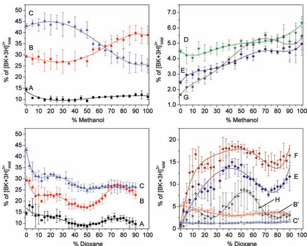
Figure 3. Peak integrations as a percent of the total [\text{BK}+3\text{H}]^{3+} distribution for the 10 labeled features in Figure 2. Percentage values for peaks A, B, C, D, E, and G are shown on top for the methanol:water solution set. Values for peaks A, B, C, F, E, and H and intermediate peaks B' and C' are shown below for the dioxane:water data set. Error bars represent the standard deviation from a triplicate analysis. Each set of points was fit with a polynomial function to illustrate change in conformer abundance as a function of solution composition.
